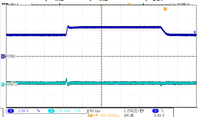
DVDD2, V_{IN1}=1.35V , V_{IN2}=3.3\sim 4.5V , I_{OUT}=1mA
