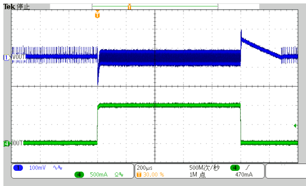
Load Transient Response VIN=5V, VO=1.8V, EN=3.6V, IO=1mA-1A
