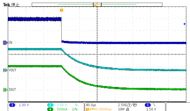
VIN=3.6V, VO=1.8V, EN=3.6V, IO=1A, EN Off
