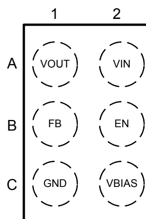
CSP-6L (Bottom View)
