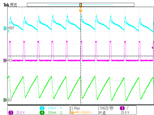
Operation Waveforms
