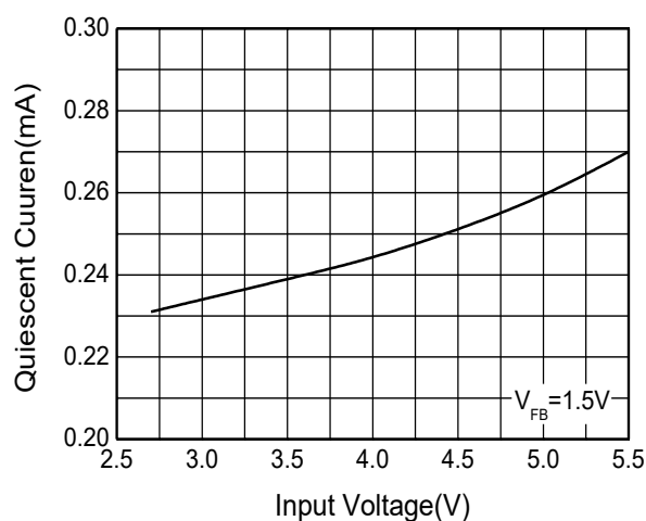
Quiescent Current vs. V_{IN}
