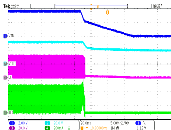
Shut-Down from VIN
