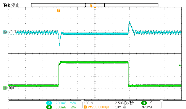
Load Transient: V_{IN}=12V, V_{EN}=5V, V_{OUT}=3.3V, I_{OUT}=0.1A-1A
